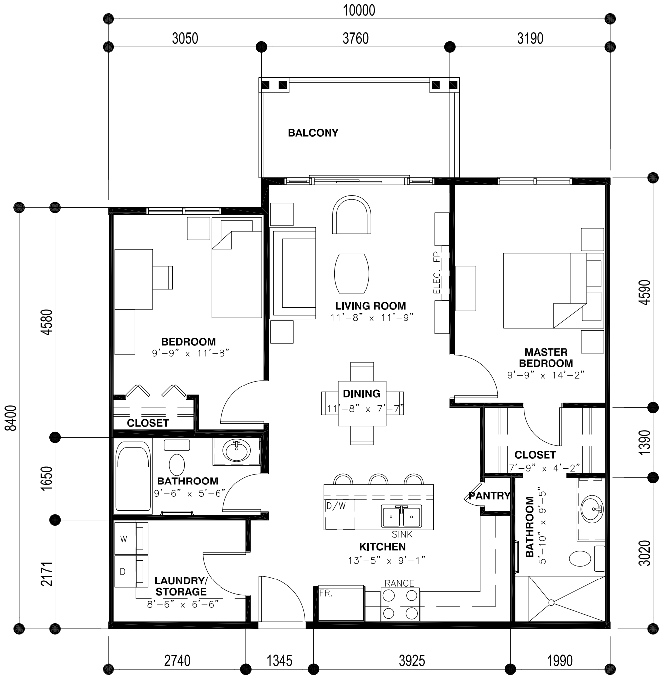
SUITE TYPE A3 (2 BEDROOM) AREA: 87.5 SQ M, 941 SQ FT
