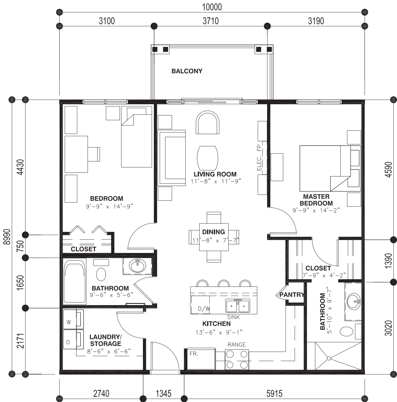
SUITE TYPE A1 (2 BEDROOM) AREA: 89.3 SQ M, 961.0 SQ FT
